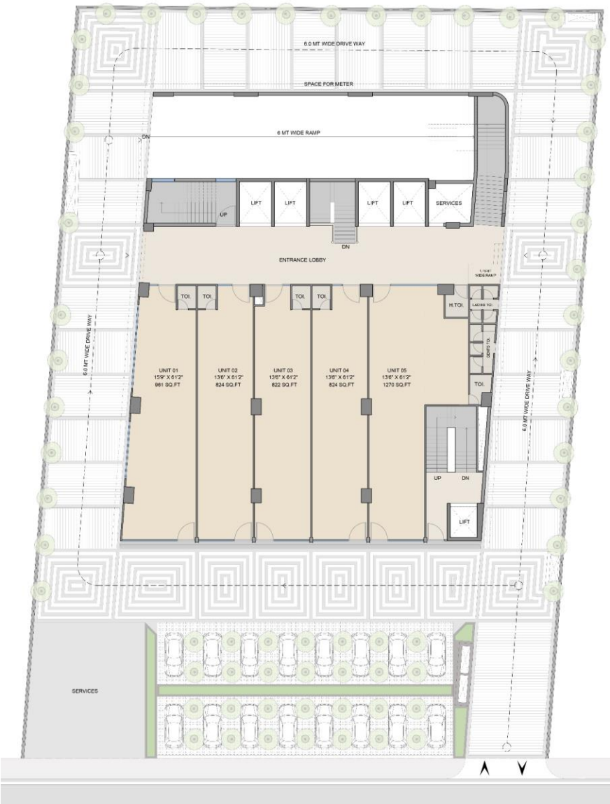
Retail : Ground and First floor Plans
