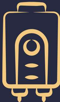
Geysers
