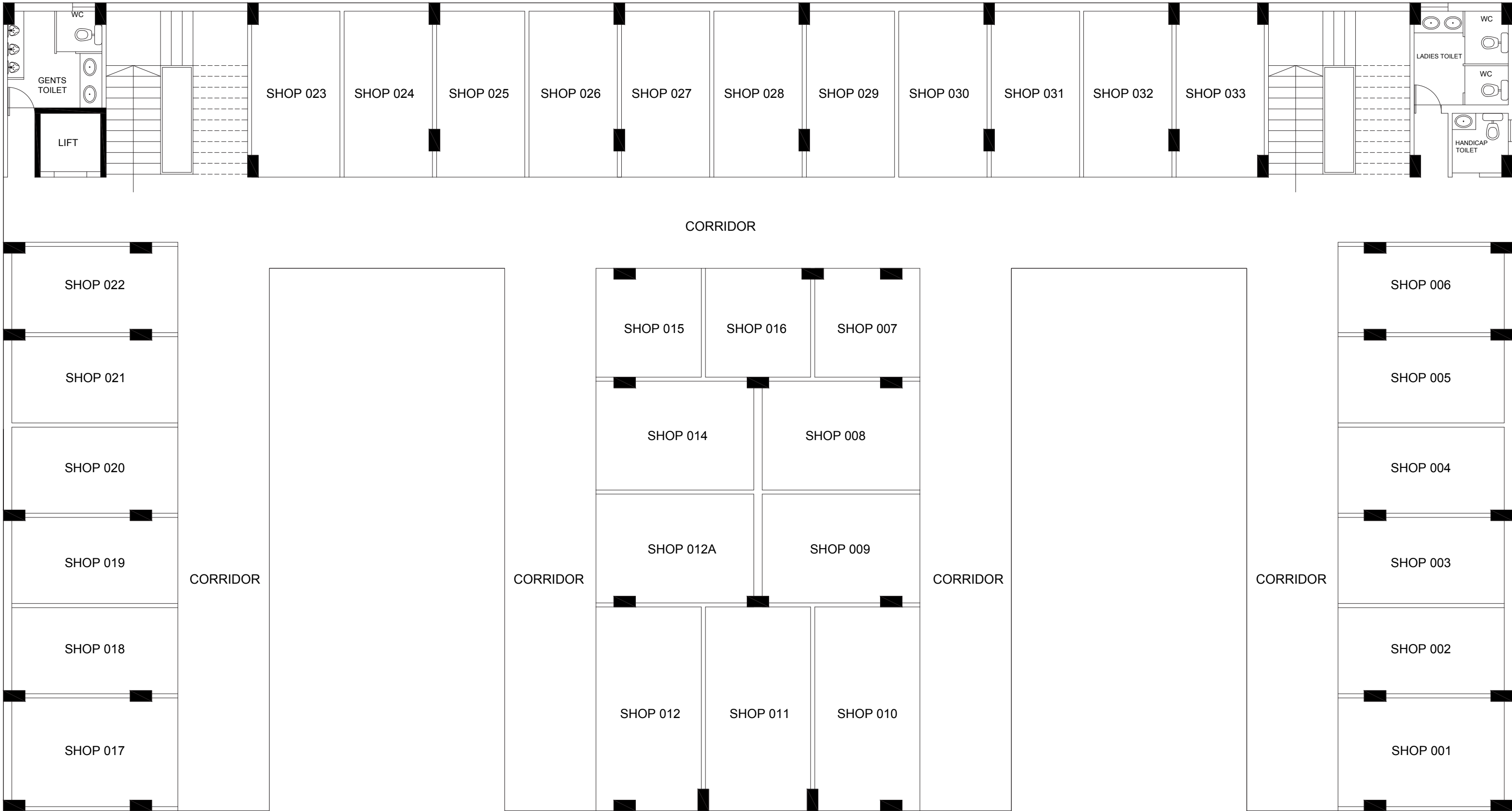
FIRST FLOOR
